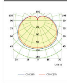
Duramax LED GL5 Dimmable 9W
