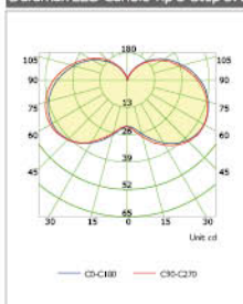
Duramax LED Candle Tip 3-Step 5W
